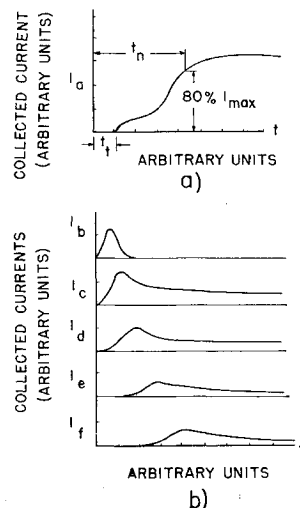
Fig. 3 Current pattern: a) on collector A; and b) on collectors B through F when the electron gun is off, and the voltage on the ionizer is applied as a step at time t = 0 .
