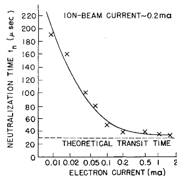
Fig. 4 Neutralization time t_n vs electron gun current for V_i = 600 \text{ v} , V_a = 200 \text{ v} , V_g = 300 \text{ v} , and V_f = 100 \text{ v} .
