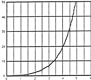
Figure 1. Graph of dimensionless spectral energy density
